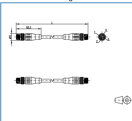
Dimensional drawing
